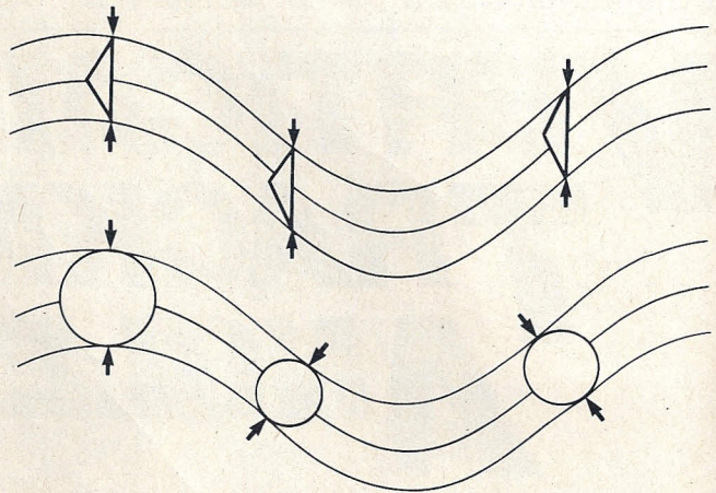
Fig. 3 — Conical stylus tracing error with lateral groove modulation, showing contact point (center of contact patch) skew relative to cutting stylus; top view.
